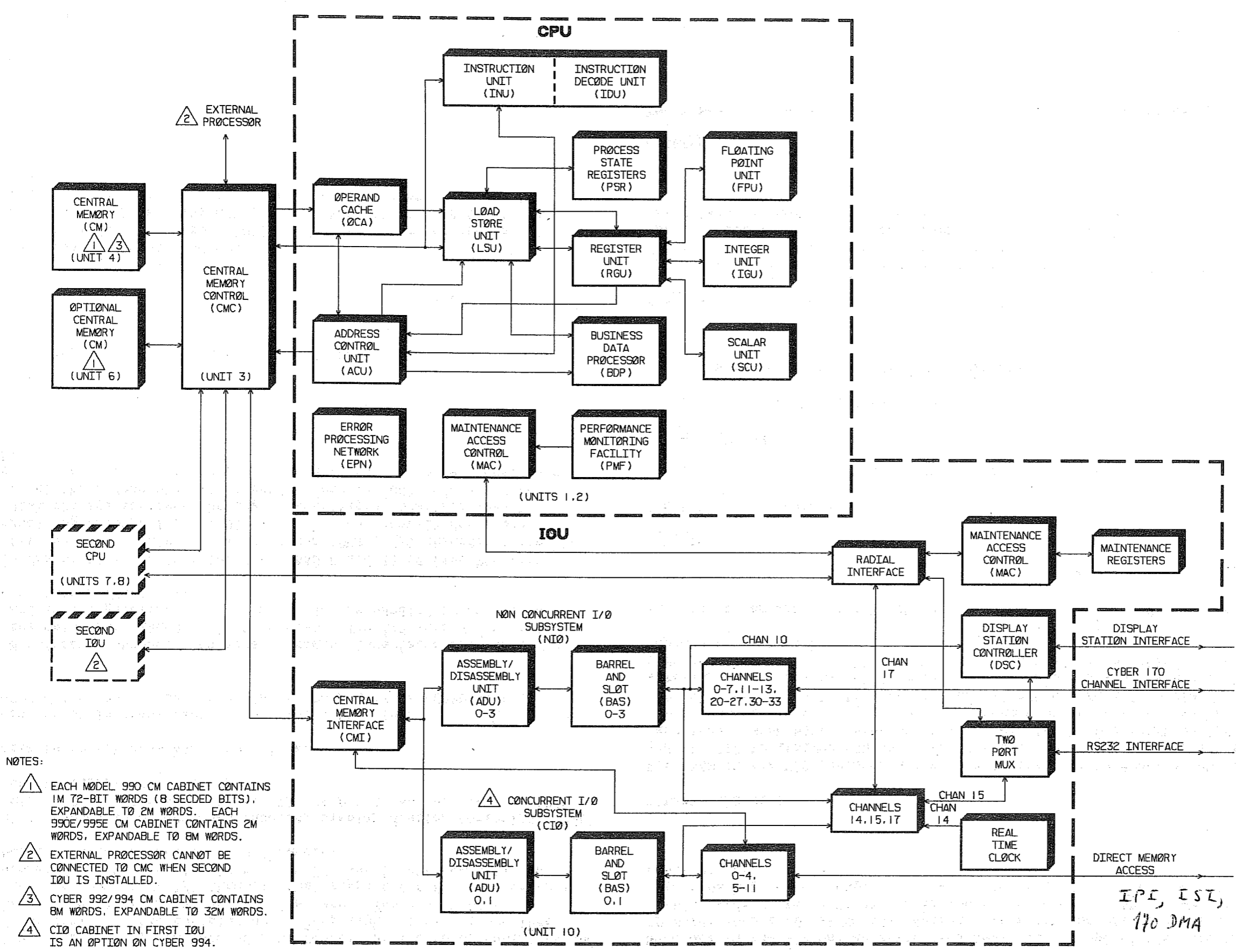
Figure 1-1. Computer System Elements
